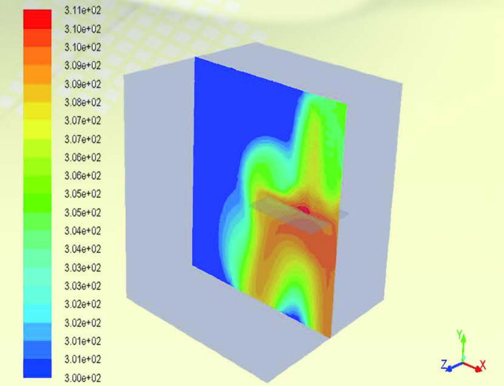
Contours of Static Temperature (K) ANSYS Fluent 15.0 (3d, pbns, ske) May 20, 2016
